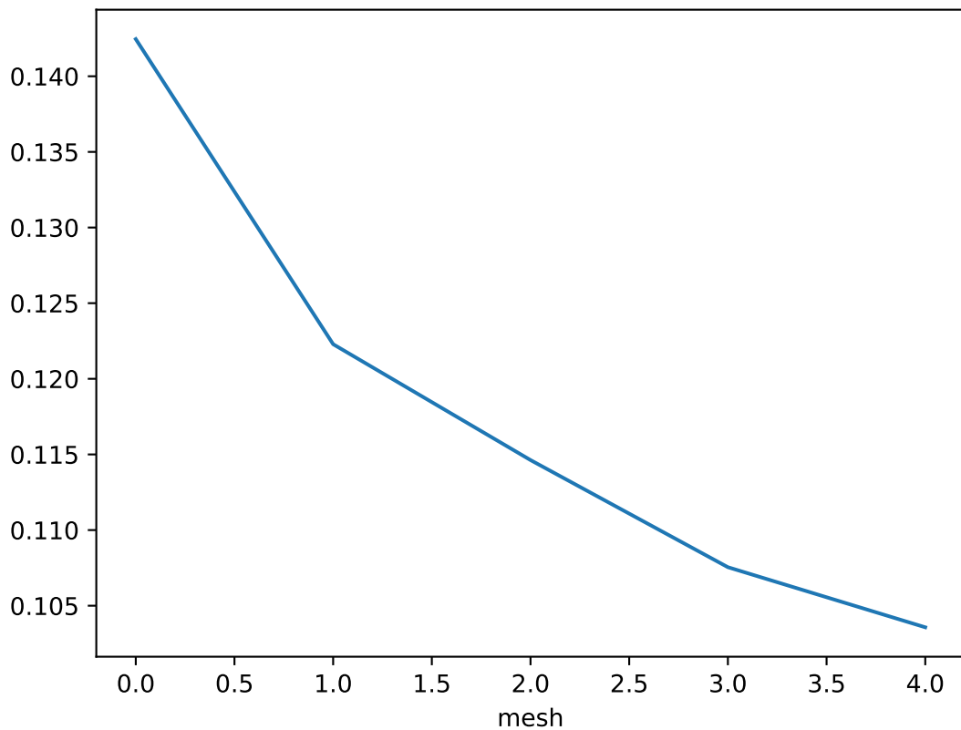
Error estimate over each mesh for z = 4.0
