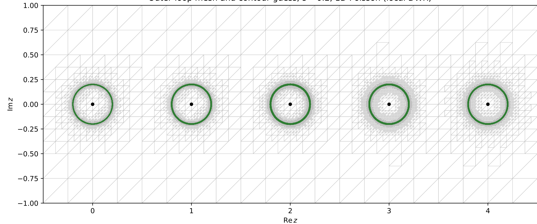
Outer-loop mesh and contour guess, \varepsilon = 0.2 , 1D Poisson (local DWR)
