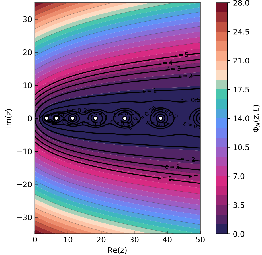
1D advection--diffusion, Hermite 3 , N = 128
