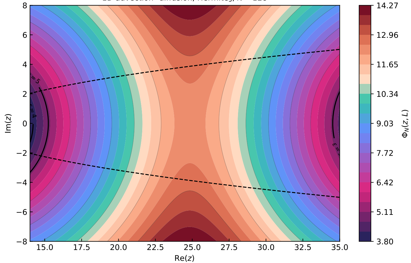
1D advection--diffusion, Hermite 3 , N = 128
