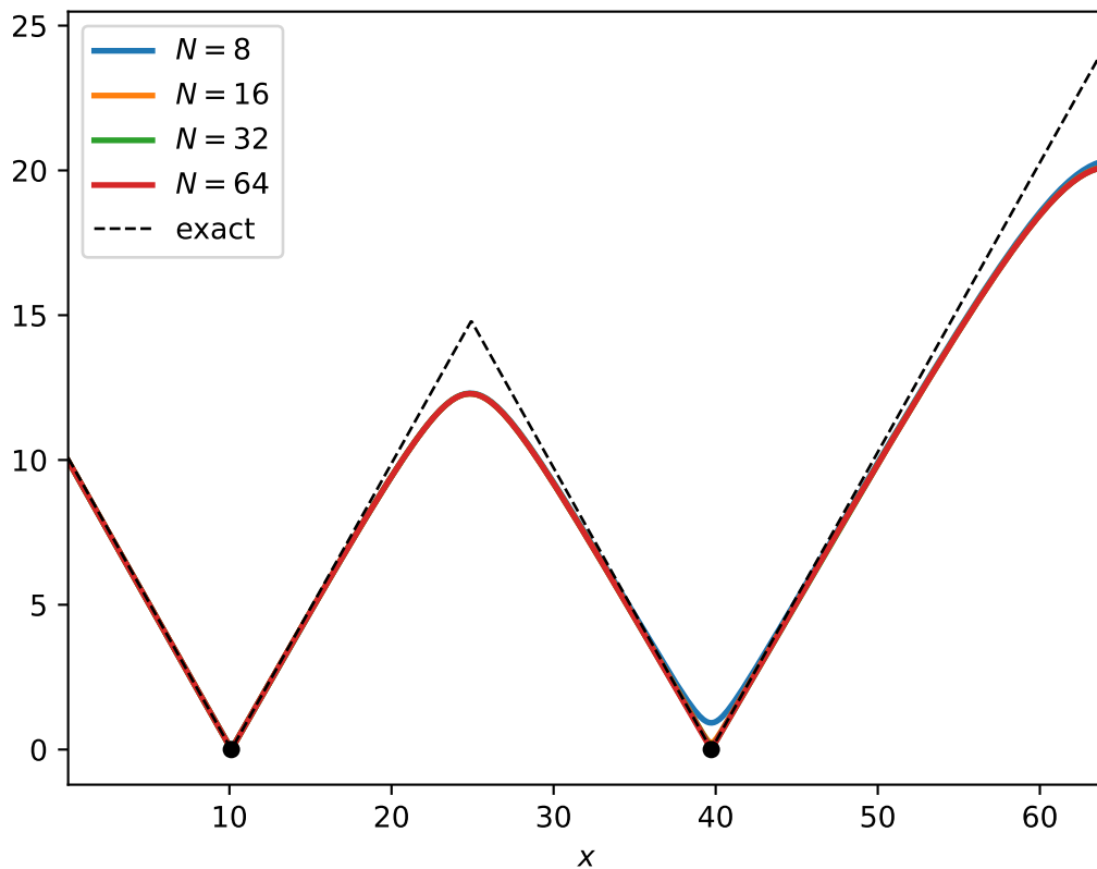
Approximation of \text{dist}(x, \text{spectrum}) , 1D Advection Diffusion (Hermite)
