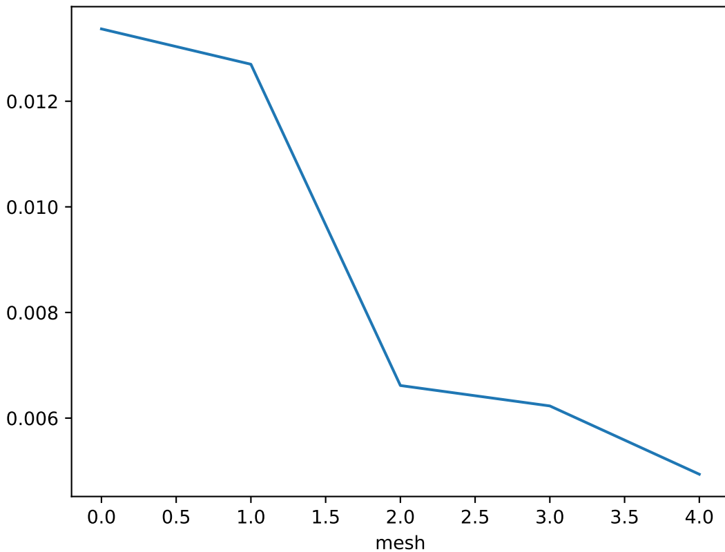
Error estimate over each mesh for z = 2.24
