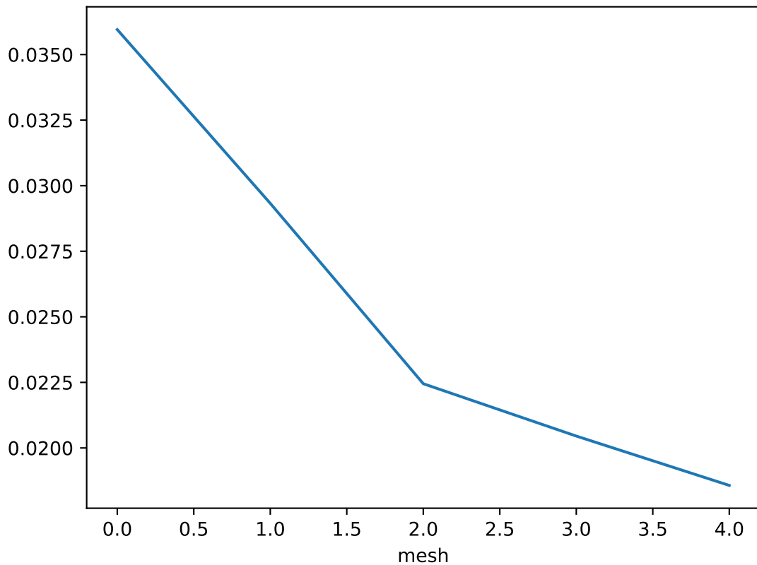
Error estimate over each mesh for z = 2.8800000000000001
