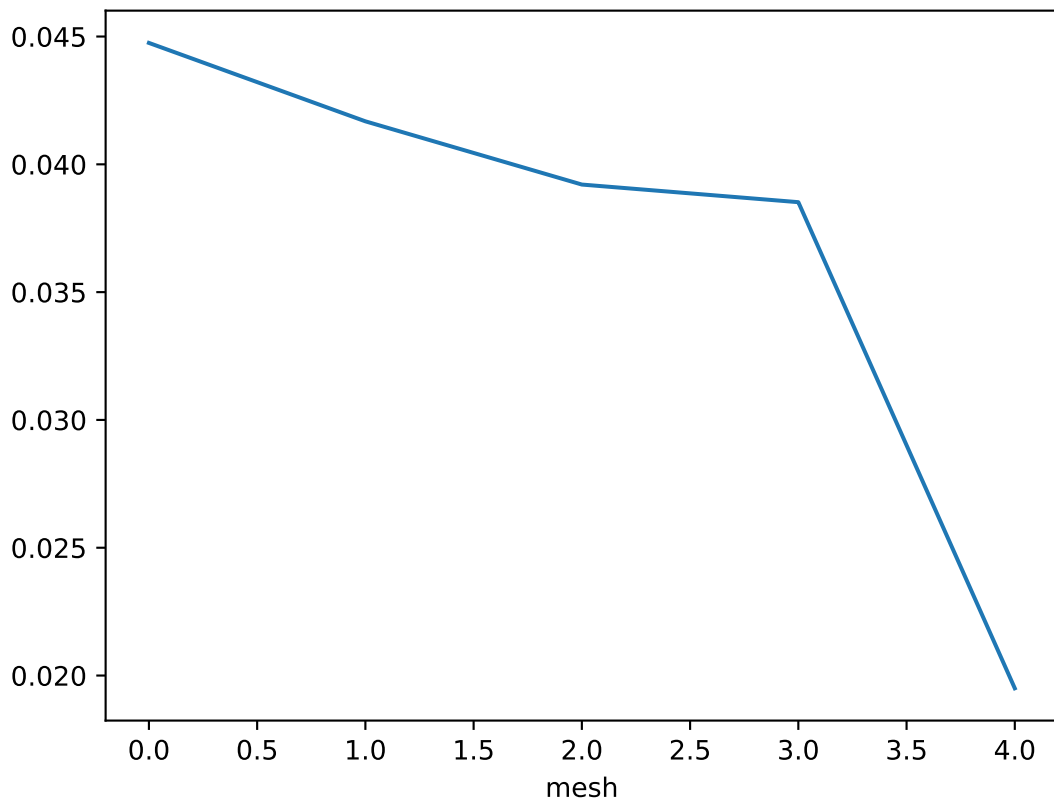
Error estimate over each mesh for z = 2.9600000000000001
