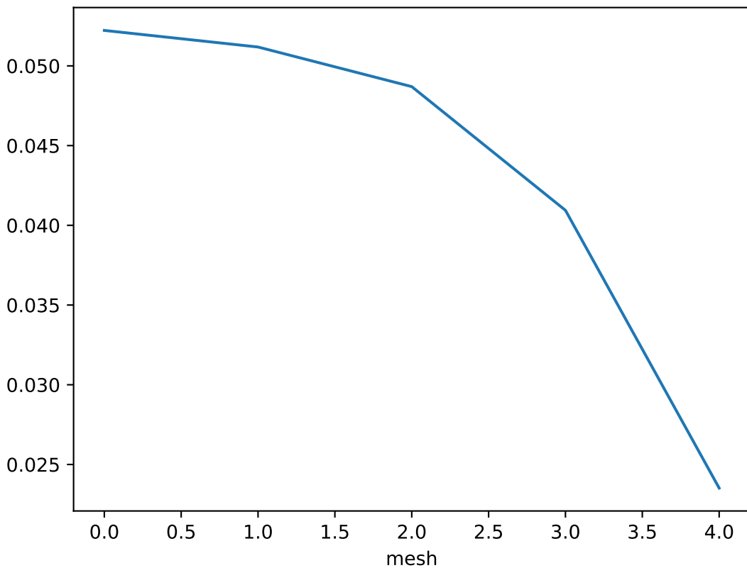
Error estimate over each mesh for z = 3.1800000000000001
