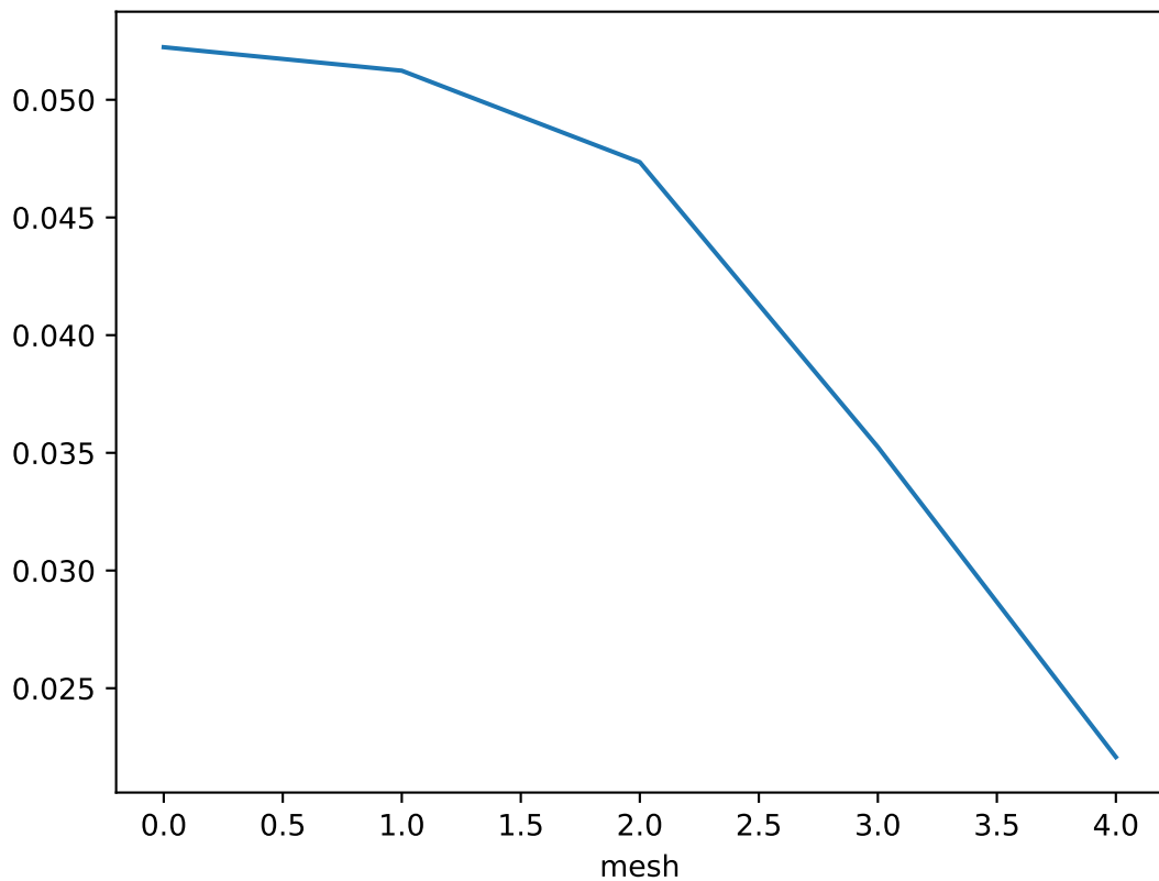
Error estimate over each mesh for z = 3.2200000000000001
