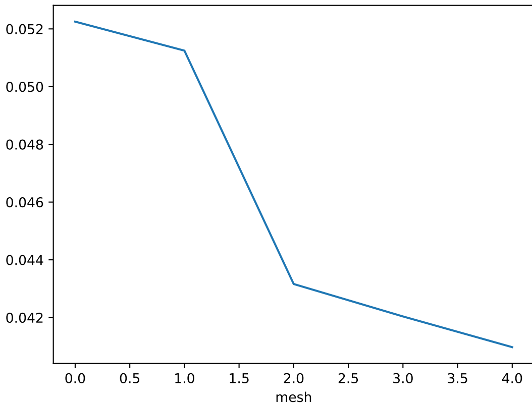
Error estimate over each mesh for z = 3.3000000000000001
