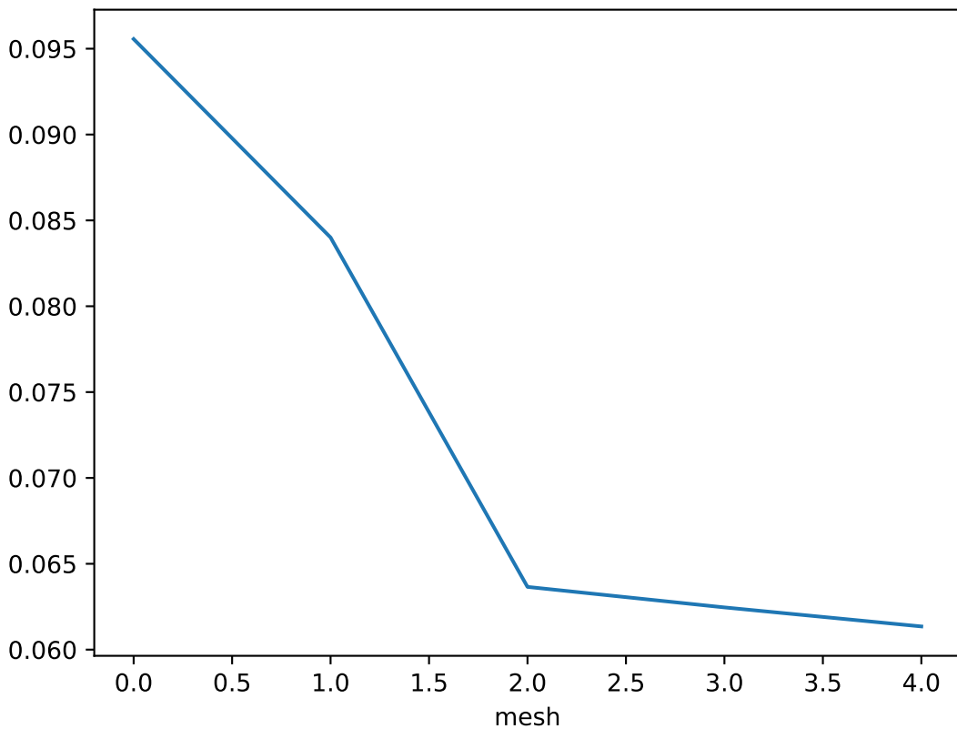
Error estimate over each mesh for z = 3.6400000000000015
