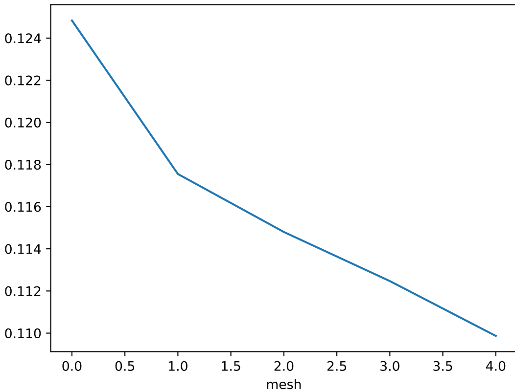
Error estimate over each mesh for z = 3.8400000000000016
