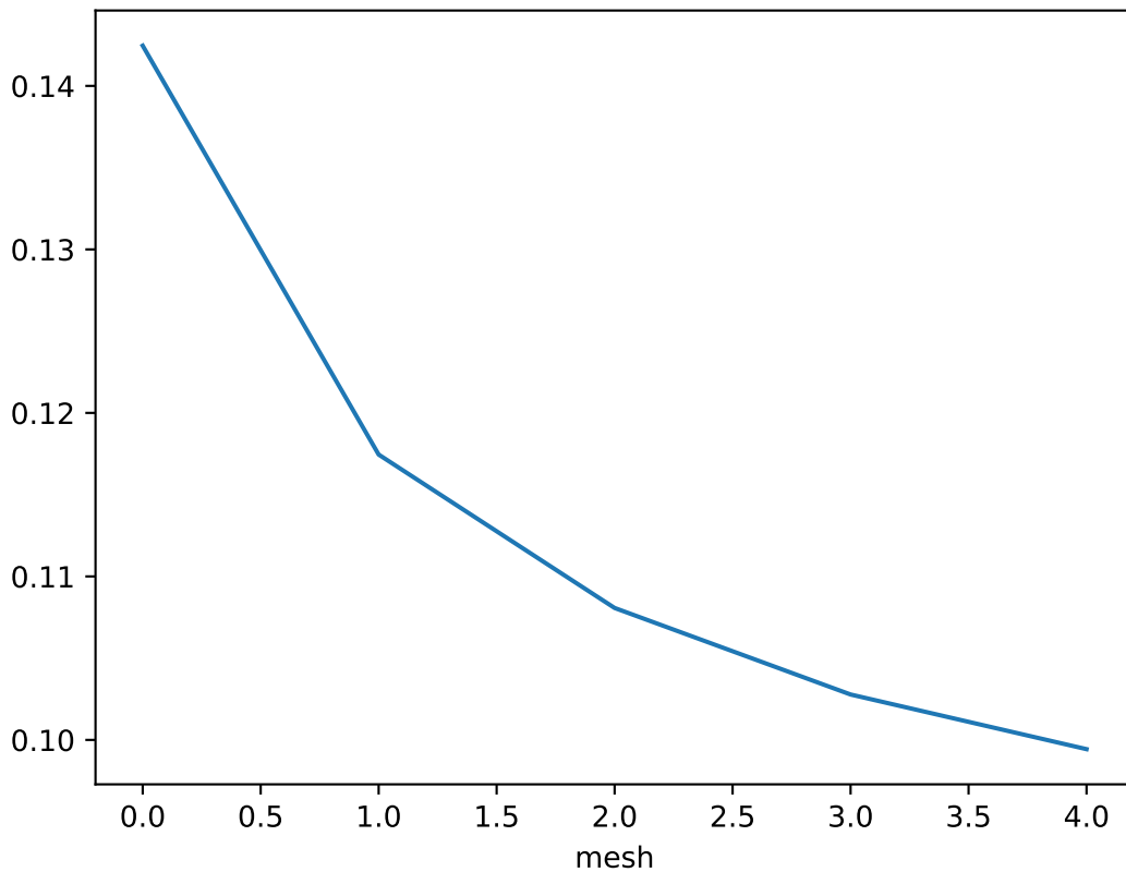
Error estimate over each mesh for z = 3.98000000000000018
