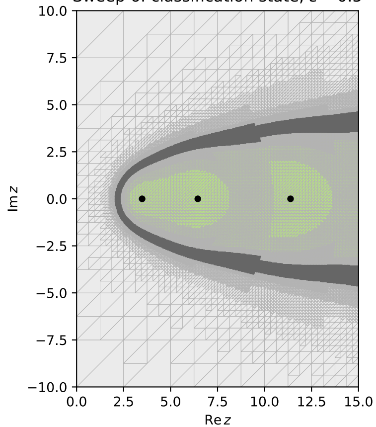
Sweep 6: classification state, \varepsilon = 0.5
