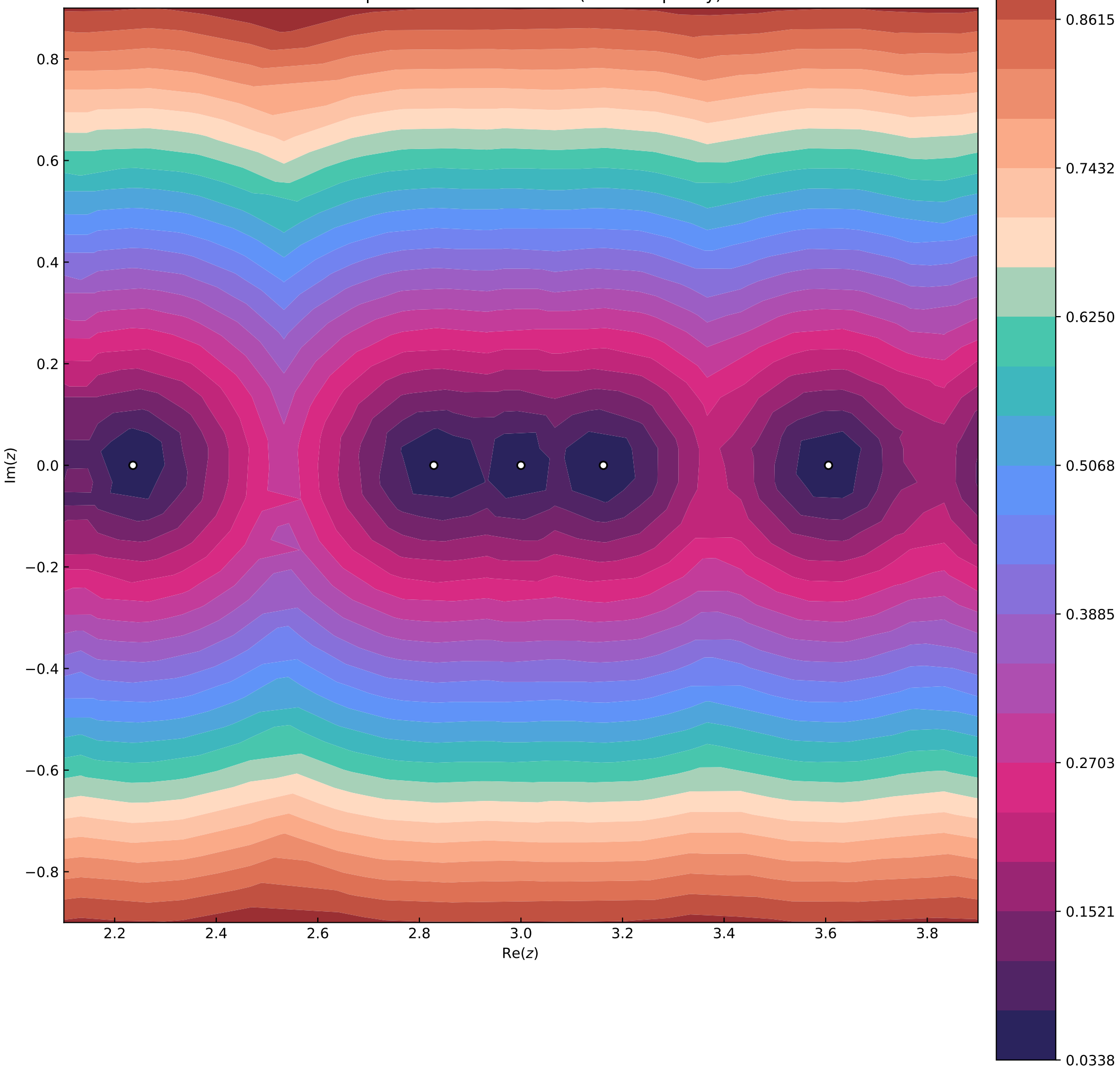
Sweep 1: DWR-corrected field (local adaptivity)
