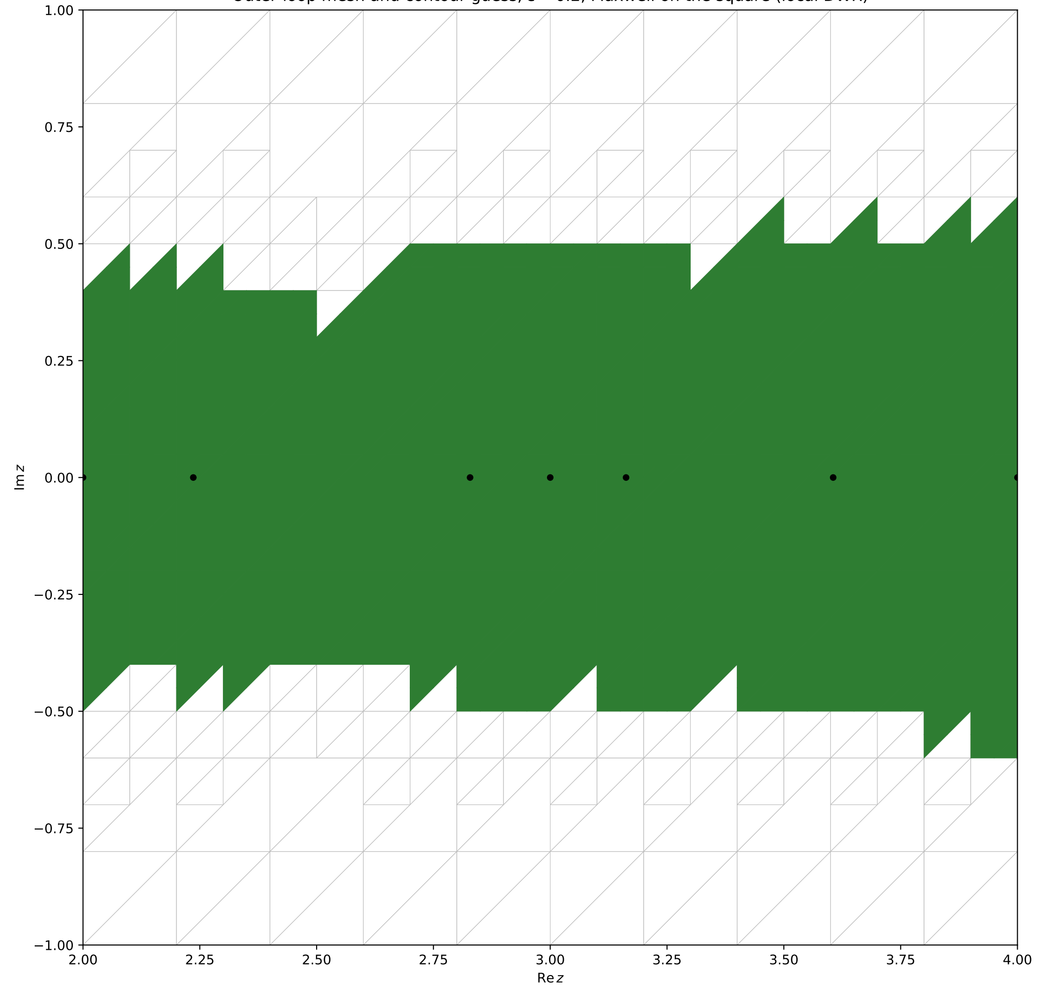
Outer-loop mesh and contour guess, \varepsilon = 0.2 , Maxwell on the square (local DWR)
