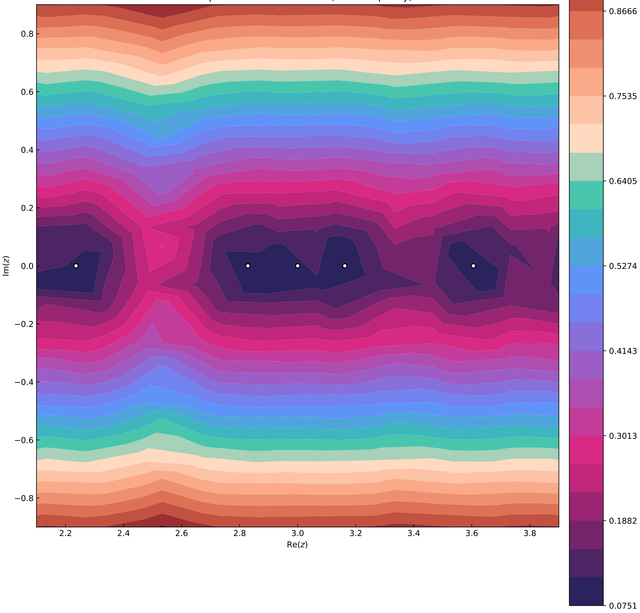
Sweep 0: DWR-corrected field (local adaptivity)
