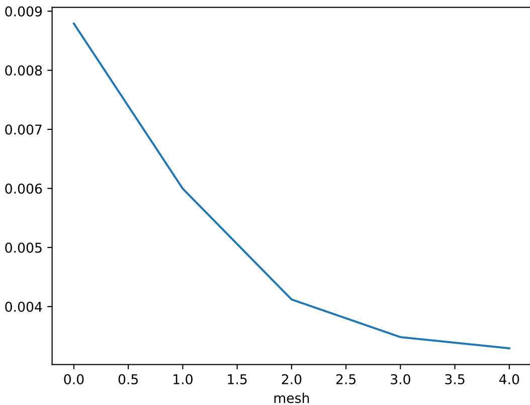
Error estimate over each mesh for z = 1.7200000000000002
