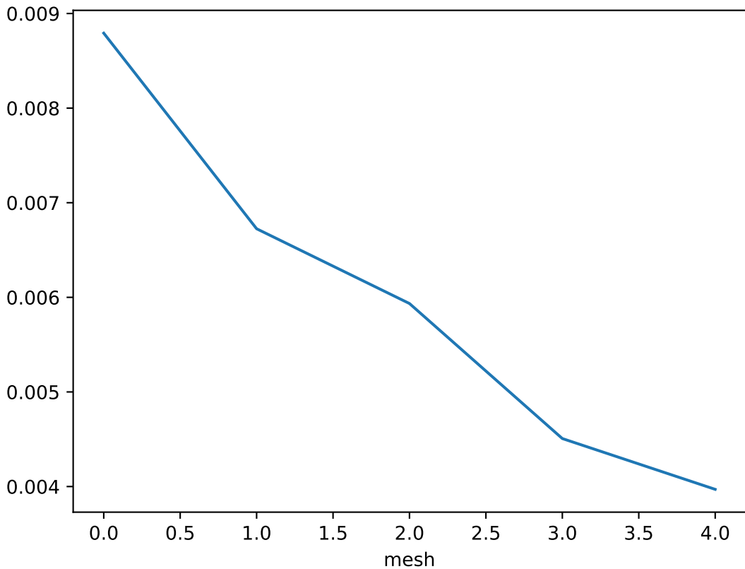
Error estimate over each mesh for z = 1.7600000000000002
