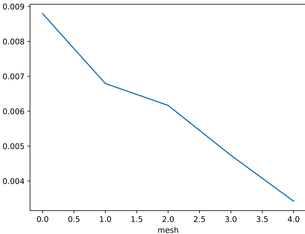
Error estimate over each mesh for z = 1.8200000000000003
