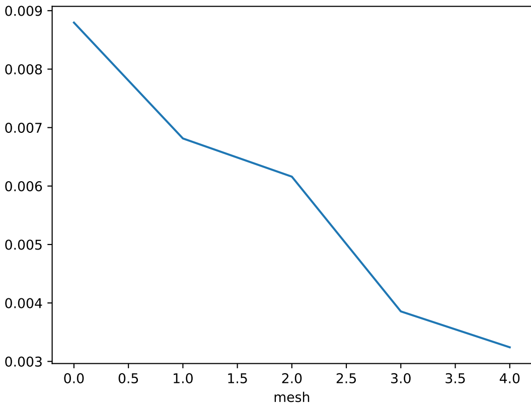
Error estimate over each mesh for z = 1.8400000000000003
