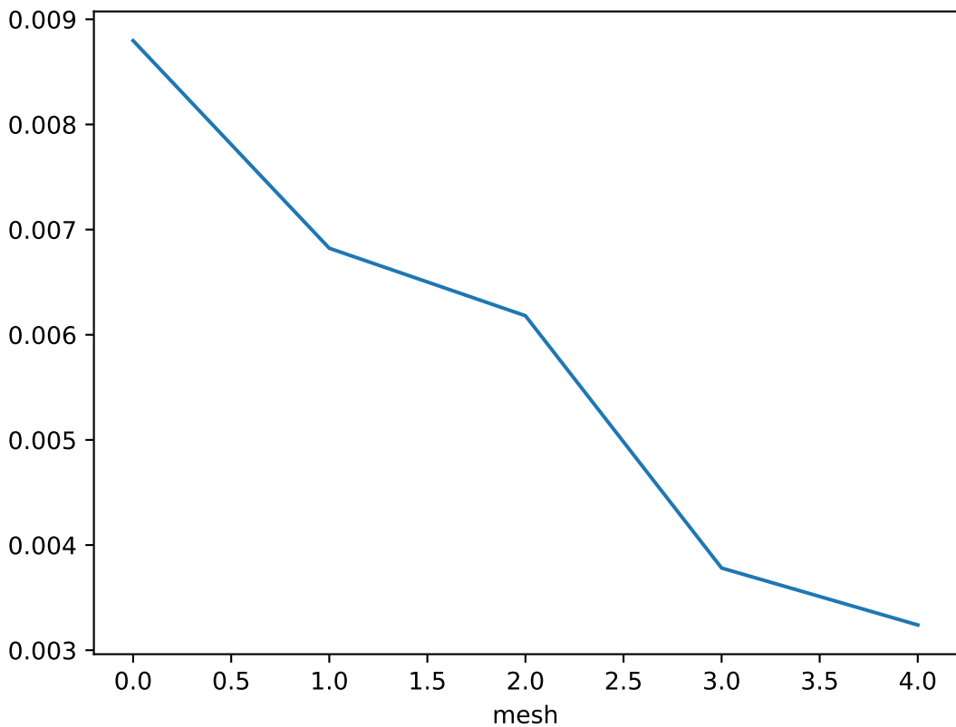
Error estimate over each mesh for z = 1.8600000000000003
