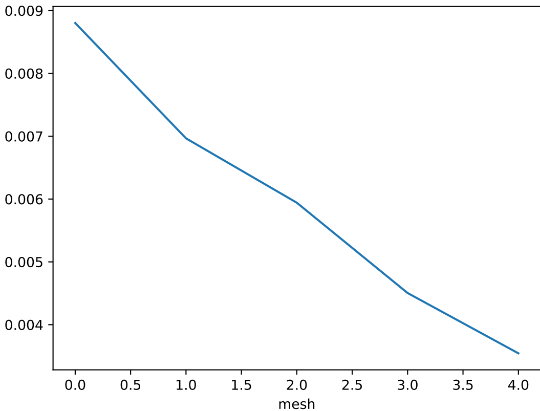
Error estimate over each mesh for z = 2.0000000000000004
