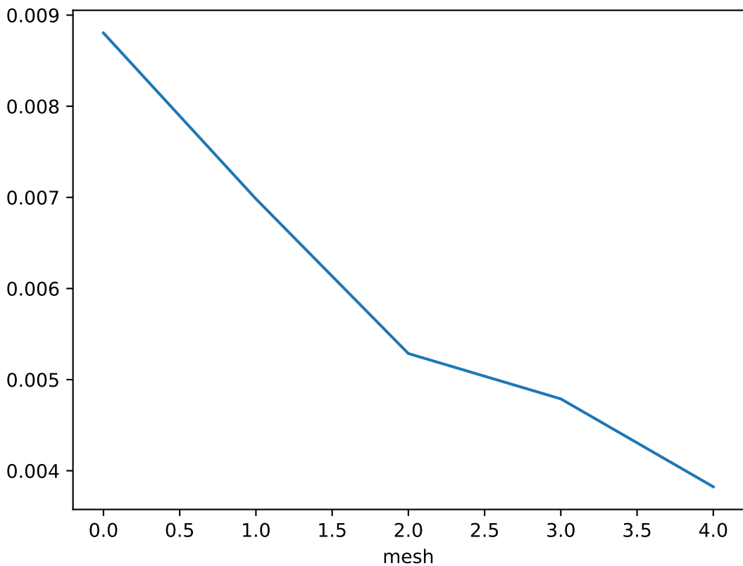
Error estimate over each mesh for z = 2.0400000000000005
