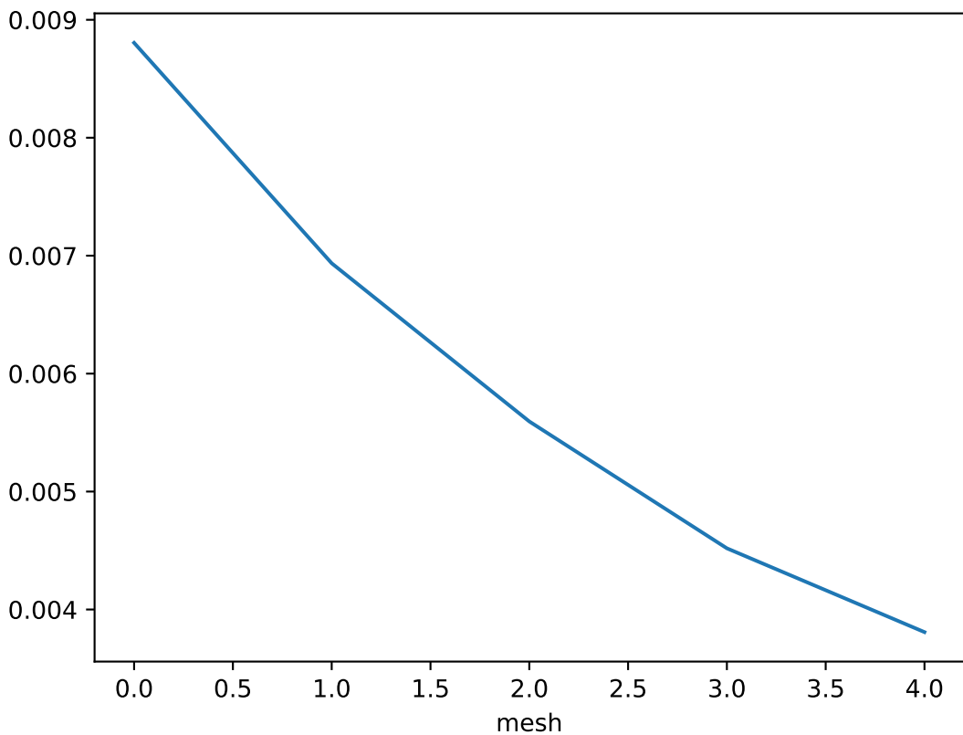
Error estimate over each mesh for z = 2.0600000000000005
