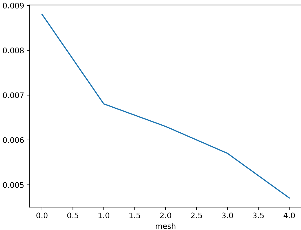
Error estimate over each mesh for z = 2.0800000000000005
