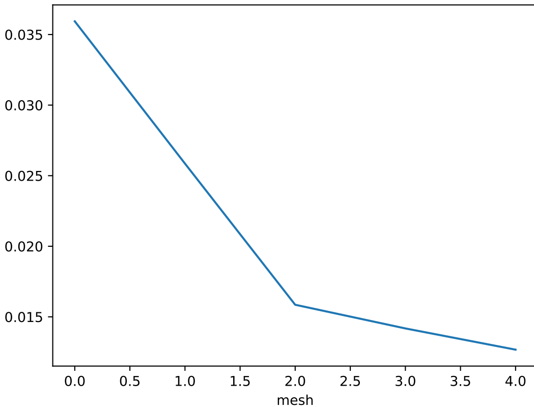
Error estimate over each mesh for z = 2.7200000000000006
