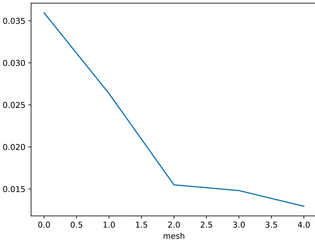
Error estimate over each mesh for z = 2.7600000000000007
