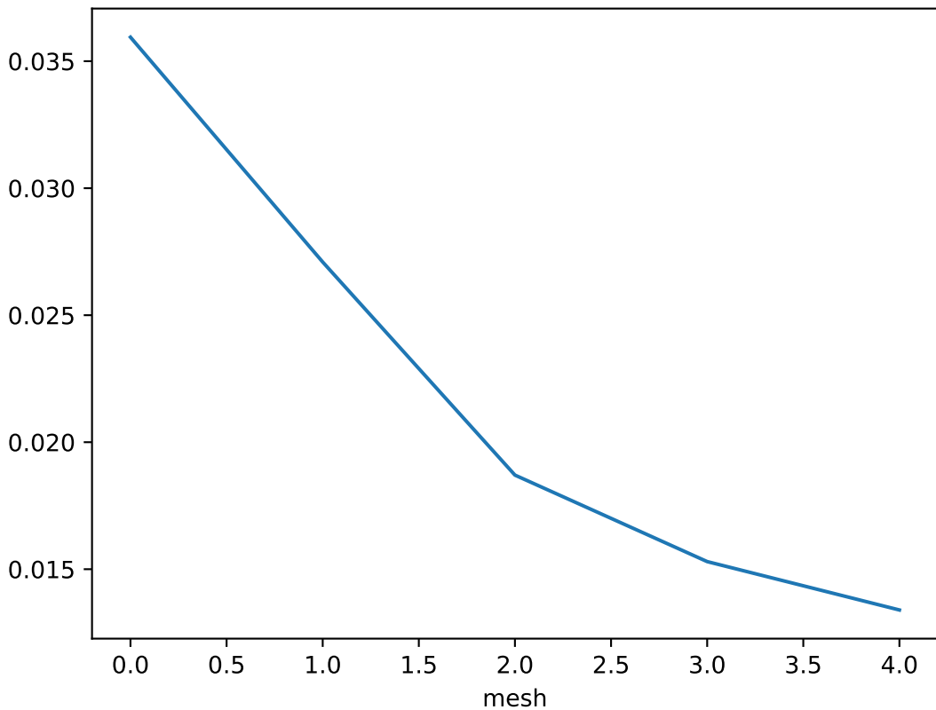
Error estimate over each mesh for z = 2.8000000000000007
