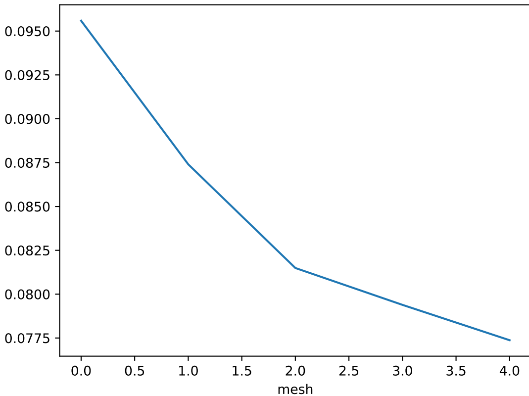
Error estimate over each mesh for z = 3.7400000000000015
