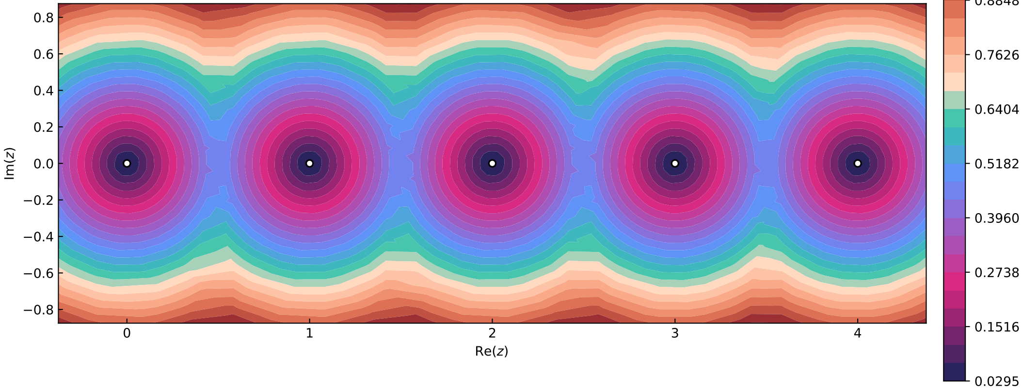
Sweep 2: DWR-corrected field (local adaptivity)
