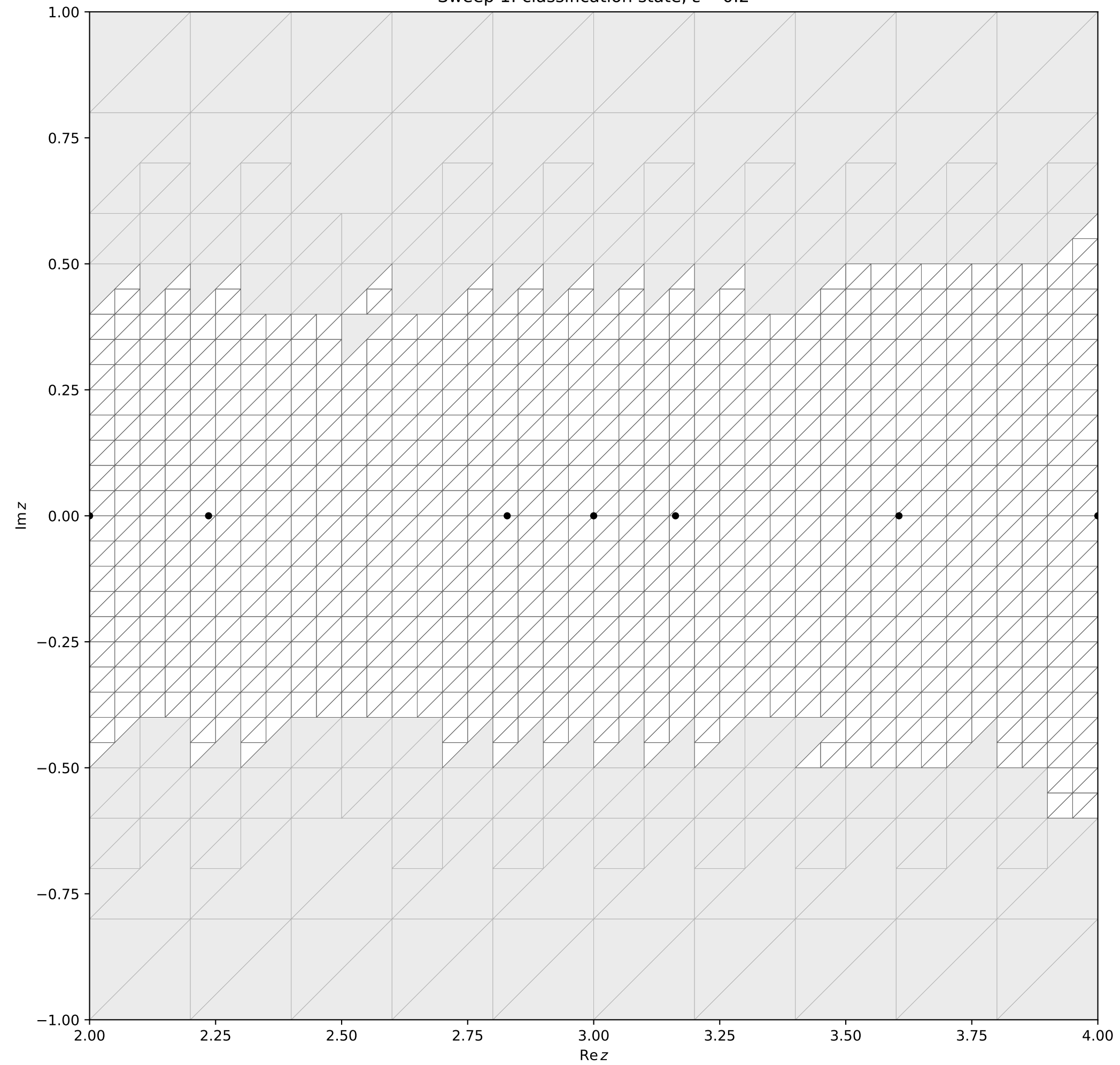
Sweep 1: classification state, \varepsilon = 0.2
