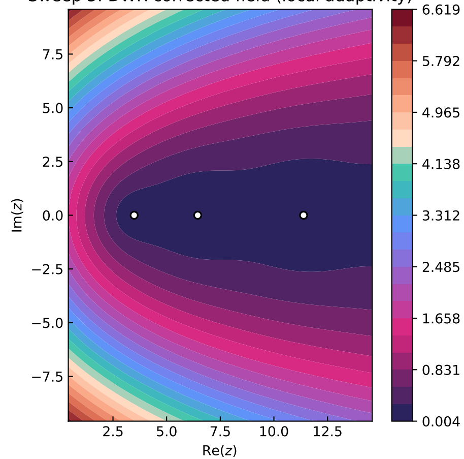
Sweep 5: DWR-corrected field (local adaptivity)
