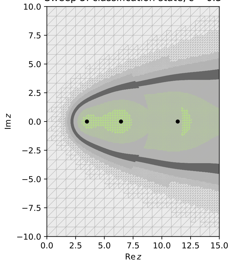
Sweep 5: classification state, \varepsilon = 0.5
