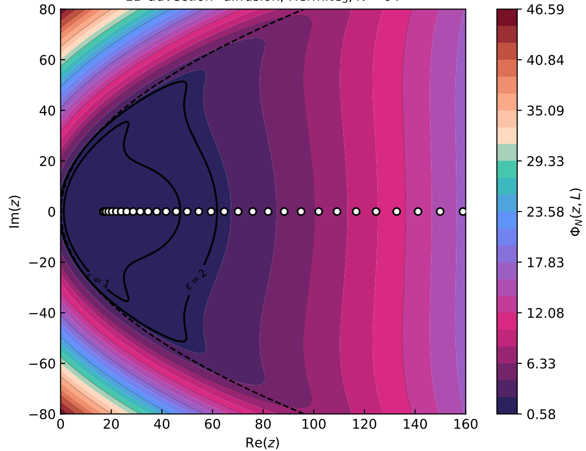
1D advection--diffusion, Hermite 3 , N = 64
