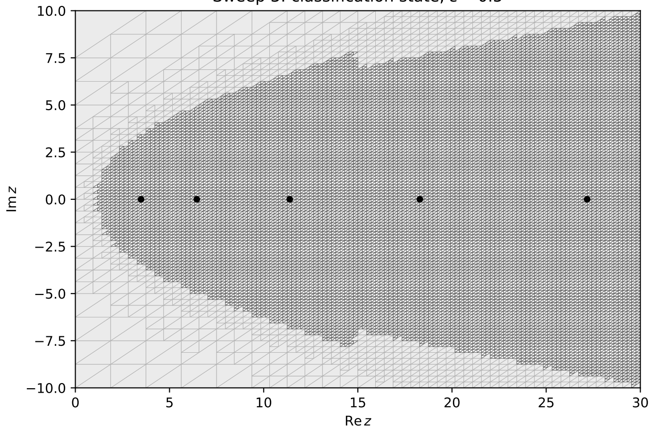
Sweep 3: classification state, \varepsilon = 0.5
