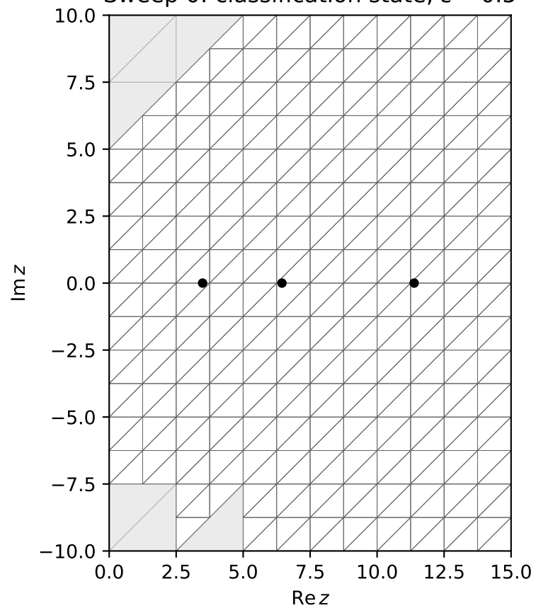
Sweep 0: classification state, \varepsilon = 0.5
