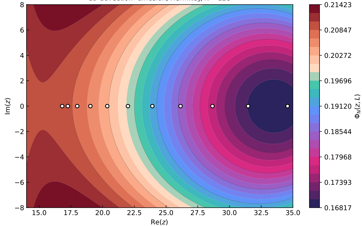
1D advection--diffusion, Hermite 3 , N = 128
