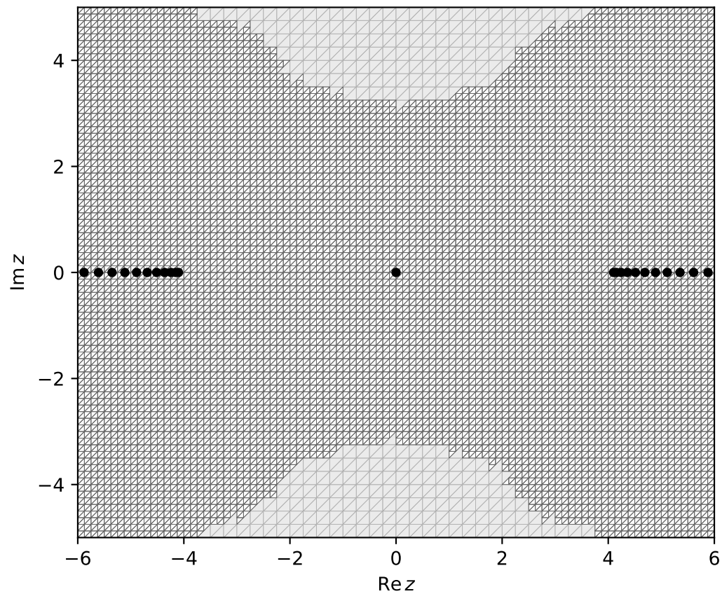
Sweep 1: classification state, \varepsilon = 0.2
