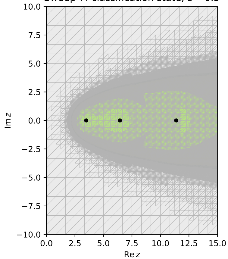
Sweep 7: classification state, \varepsilon = 0.5
