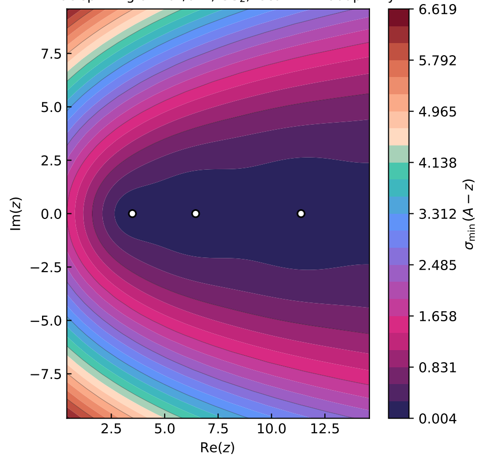
Dirac splitting of -\mathrm{d}^2/\mathrm{d}x^2 , CG 2 , local DWR adaptivity
