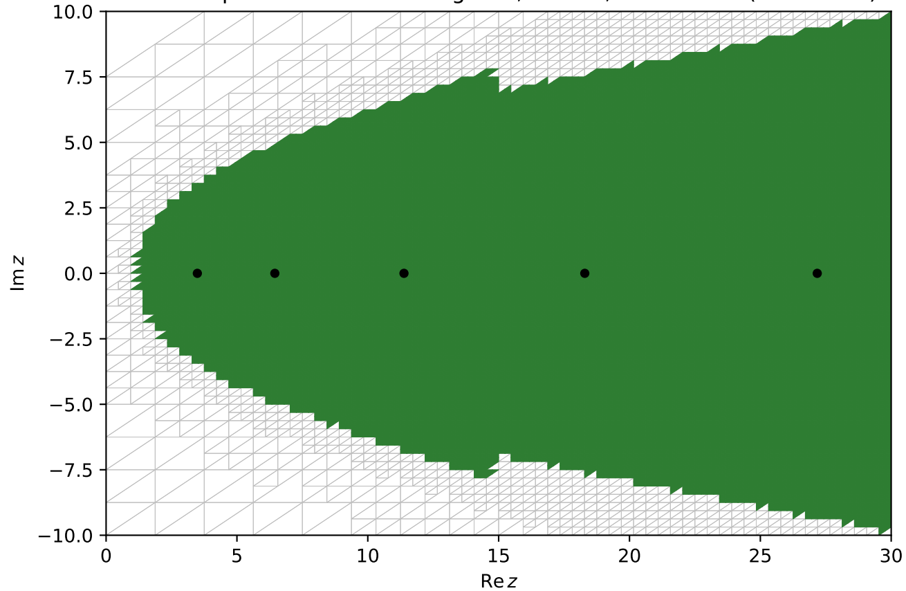
Outer-loop mesh and contour guess, \varepsilon = 0.5 , 1D Poisson (local DWR)
