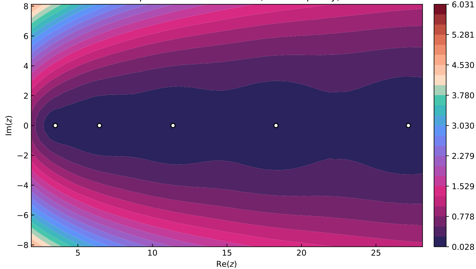
Sweep 2: DWR-corrected field (local adaptivity)
