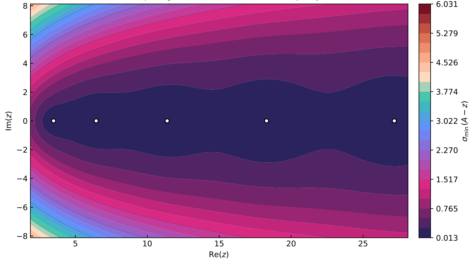
Dirac splitting of -d^2/dx^2 , CG 2 , local DWR adaptivity
