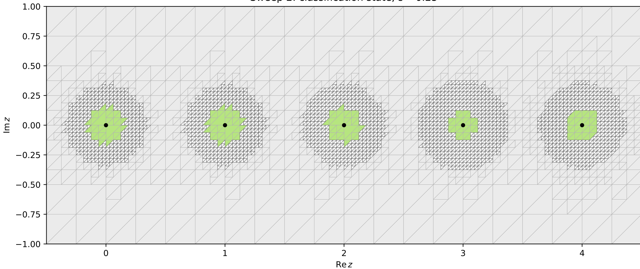
Sweep 2: classification state, \varepsilon = 0.25
