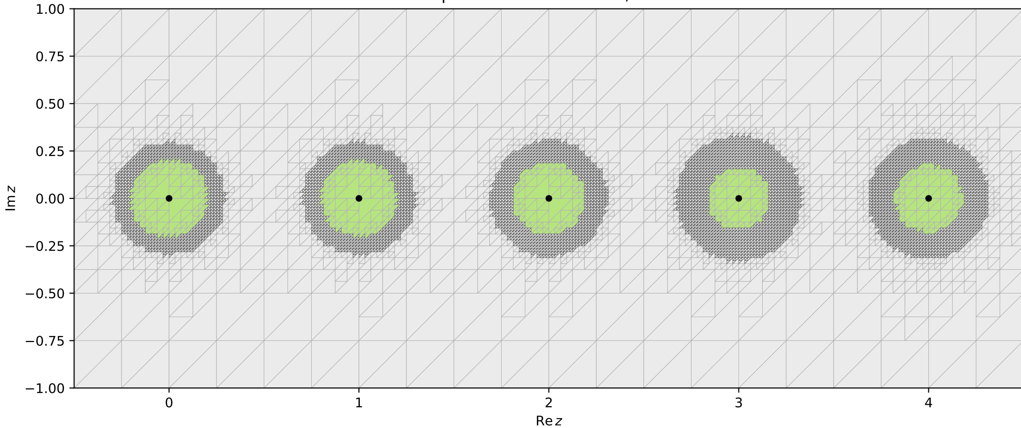
Sweep 3: classification state, \varepsilon = 0.25
