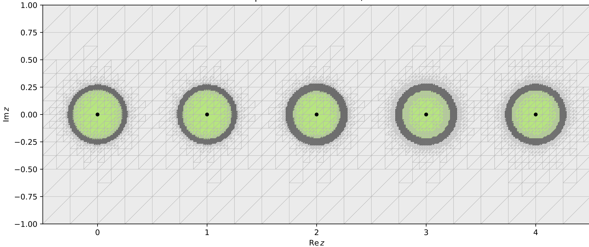
Sweep 4: classification state, \varepsilon = 0.25
