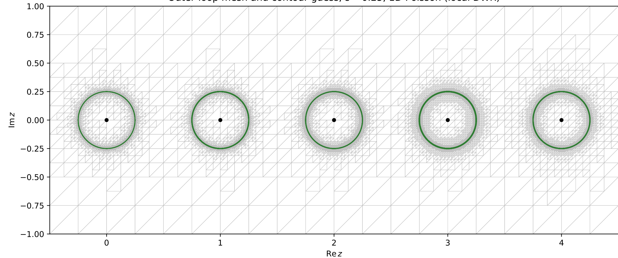
Outer-loop mesh and contour guess, \varepsilon = 0.25 , 1D Poisson (local DWR)
