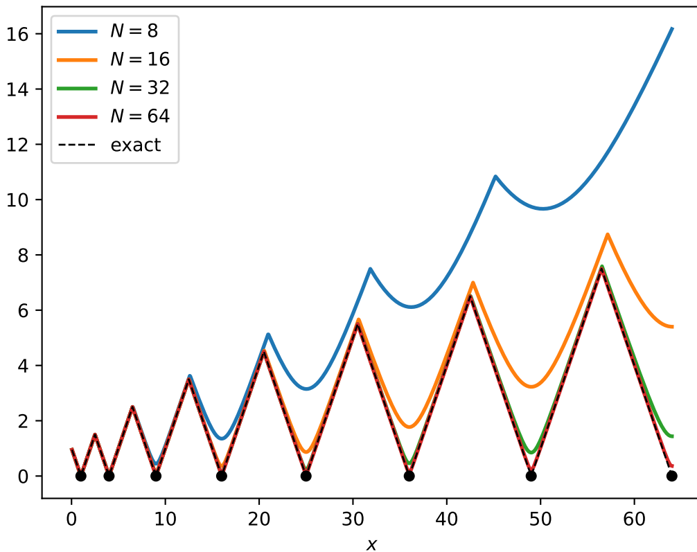
Approximation of \text{dist}(x, \text{spectrum}) , 1D Poisson (Hermite)
